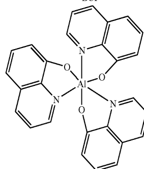
\text{Alq}_3
