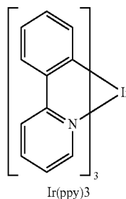
\text{Ir(ppy)}_3
